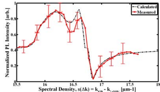
Fig 2. A QW PL emission at 820nm illustrating a match in calculated and measured in [1] intensity modulation.
